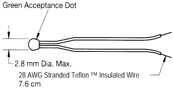
Type T Lead Configuration
