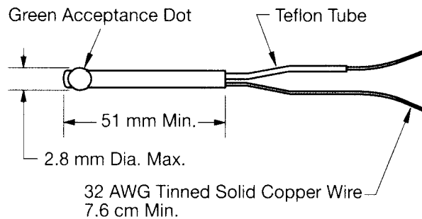
Type E Lead Configuration
