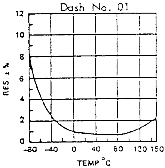
Figure 2. Resistance tolerance curves (Page 1 of 2).
