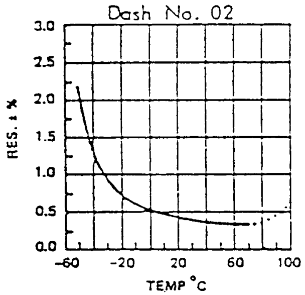
Figure 2. Resistance tolerance curves (Page 1 of 2).
