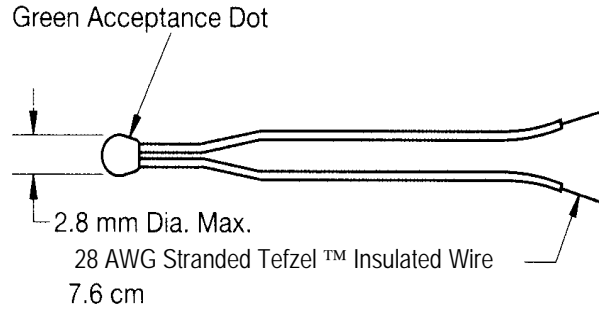
Type A Lead Configuration
