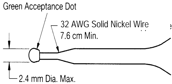
Type N Lead Configuration
