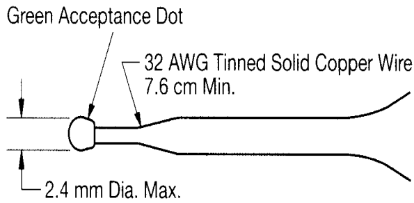
Type S Lead Configuration
